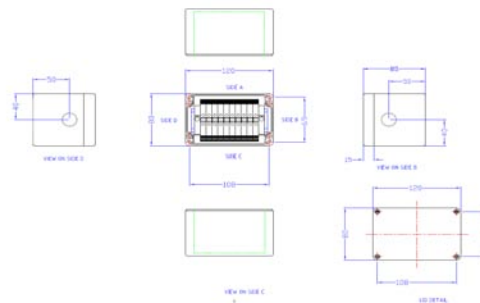
JB-FT10 Drawing
