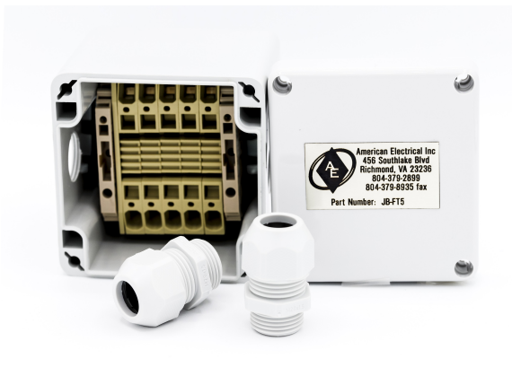
5 Terminals
